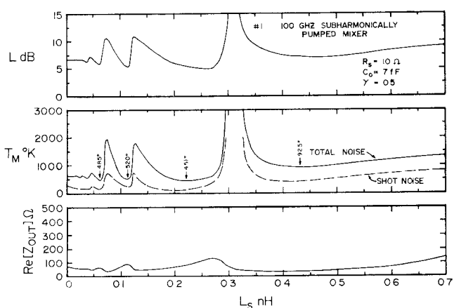
Fig. 4. Example 1: 100-GHz subharmonically pumped mixer of Fig. 1 with Z_3=0 for all frequencies beyond the signal and image, \omega_{\pm 2} . The conversion loss and equivalent input noise temperature, both SSB, and real part of the IF output impedance, are shown as functions of inductance L_S . Other details are given in Table I.
