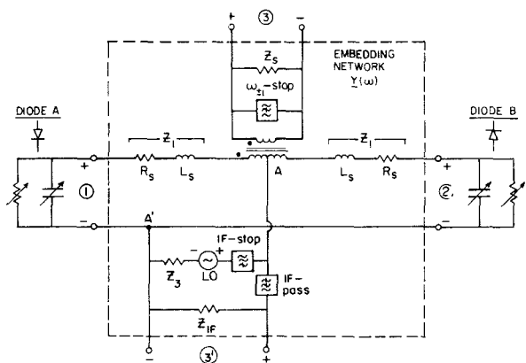
Fig. 2. Circuit of the balanced mixer used in examples 5 and 6. The diodes are connected with opposite polarity so they conduct on alternate half-cycles of the LO. The series resistance R_s of the diodes is considered part of the embedding network. Z_s is the source impedance at the signal and image frequencies \omega_{\pm 1} , and Z_3 is the LO source impedance. Because of the symmetry of the circuit, Z_3 is seen only by odd LO harmonics and even-order sidebands \omega_{\pm 2}, \omega_{\pm 4} , etc. Z_{IF} is the IF load impedance which is conjugate-matched to the output impedance of the mixer.
